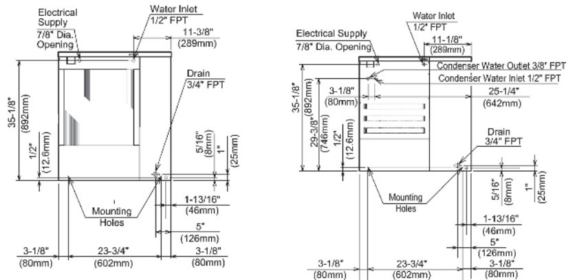
AIR-COOLED UNIT
