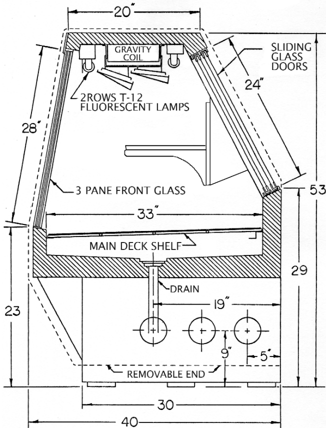
Cross Section
