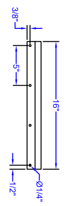
MOUNTING BRACKET
