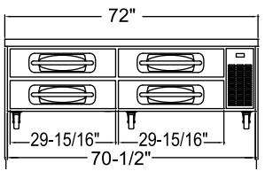
KSCB72 ELEVATION VIEW
