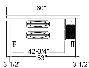
KSCB60 ELEVATION VIEW
