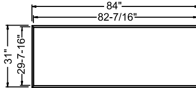
KSCB84 PLAN VIEW
