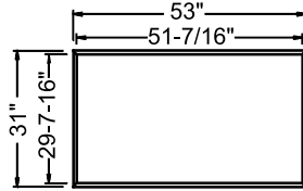
KSCB53 PLAN VIEW
