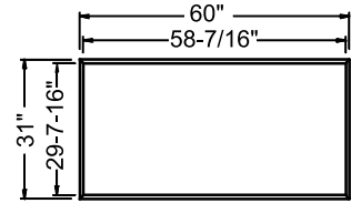
KSCB60 PLAN VIEW
