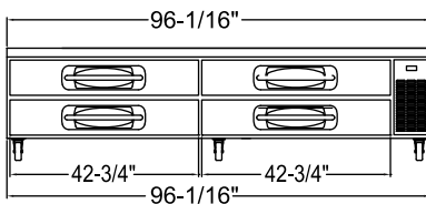
KSCB96 ELEVATION VIEW
