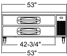
KSCB53 ELEVATION VIEW
