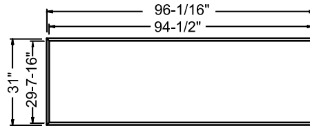
KSCB96 PLAN VIEW
