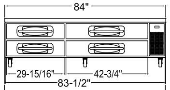
KSCB84 ELEVATION VIEW
