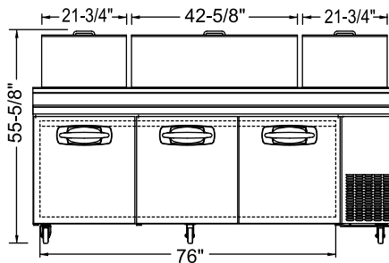
KSPT93 ELEVATION VIEW
