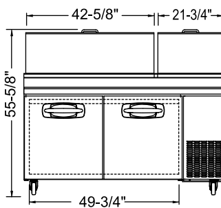
KSPT67 ELEVATION VIEW
