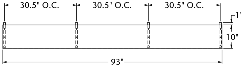
PLAN VIEW KSPT93
