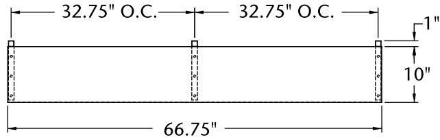
PLAN VIEW KSPT67
