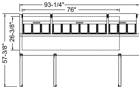
KSPT93 PLAN VIEW
