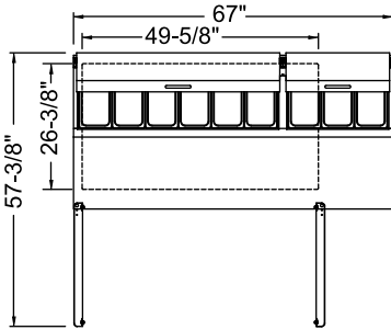
KSPT67 PLAN VIEW
