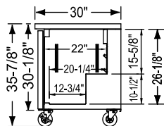
KSUR/KSUF48 ELEVATION VIEW
