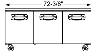
KSUR72 ELEVATION VIEW
