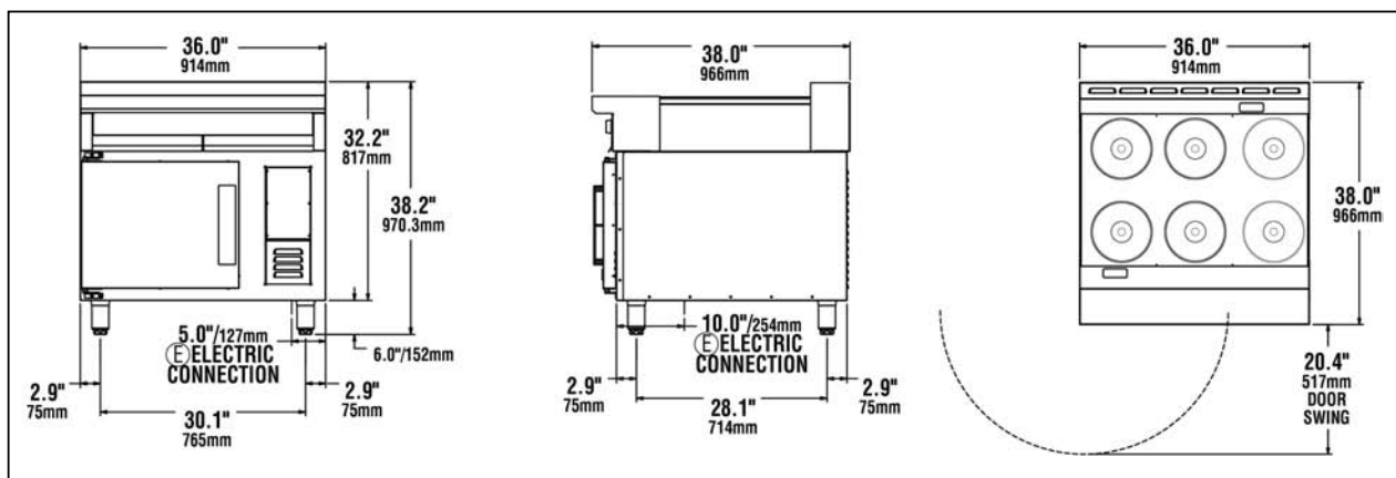
[Front View/Elevation]
