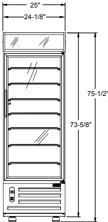
ELEVATION VIEW
