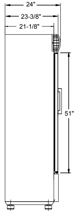
SIDE VIEW
