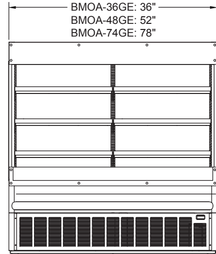
ELEVATION VIEW
