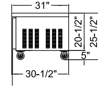
SIDE VIEW - ALL MODELS
