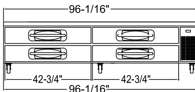
MBCB96 ELEVATION VIEW
