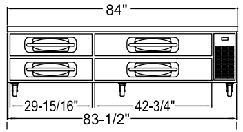
MBCB84 ELEVATION VIEW
