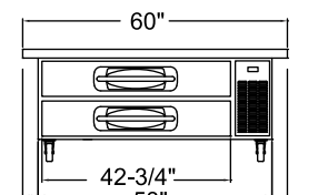
MBCB60 ELEVATION VIEW
