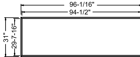
MBCB96 PLAN VIEW
