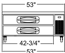
MBCB53 ELEVATION VIEW
