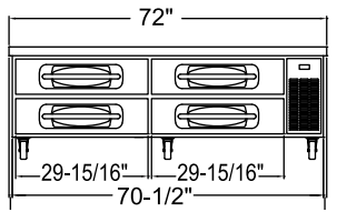
MBCB72 ELEVATION VIEW
