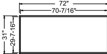
MBCB72 PLAN VIEW
