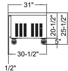
SIDE VIEW - ALL MODELS
