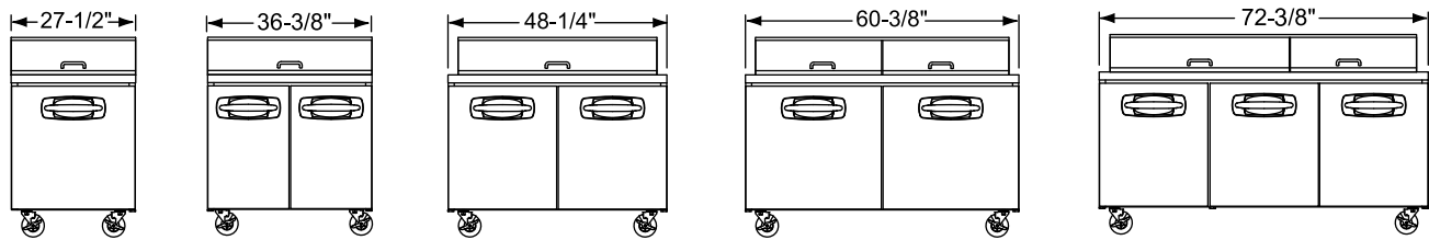
MBSMP27-12 ELEVATION VIEW
