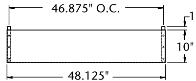
PLAN VIEW MBUR/MBUF48A
