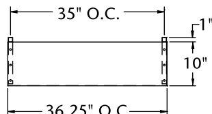
PLAN VIEW MBUR36A
