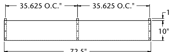
PLAN VIEW MBUR72A
