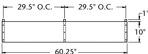
PLAN VIEW MBUR/MBUF60A
