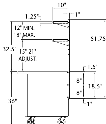
DOUBLE SHELF SIDE VIEW
