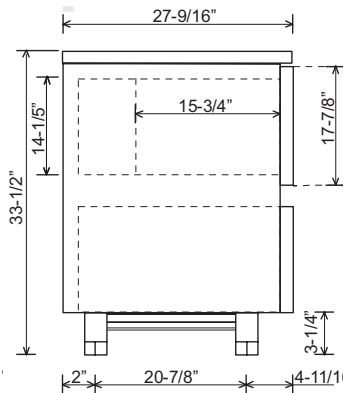
NBC40-4 - Side Views
