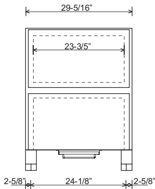
NBC40-4 - Front Views
