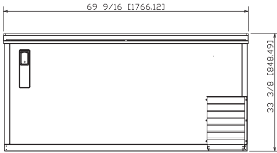
FRONT NLBC69
