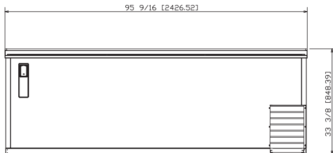
FRONT NLBC95
