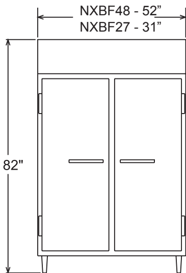
ELEVATION VIEW
