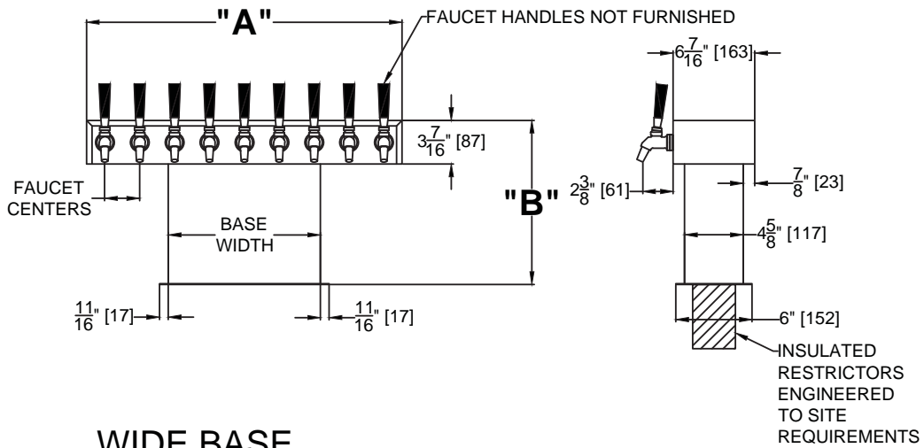
WIDE BASE TEE TOWERS
