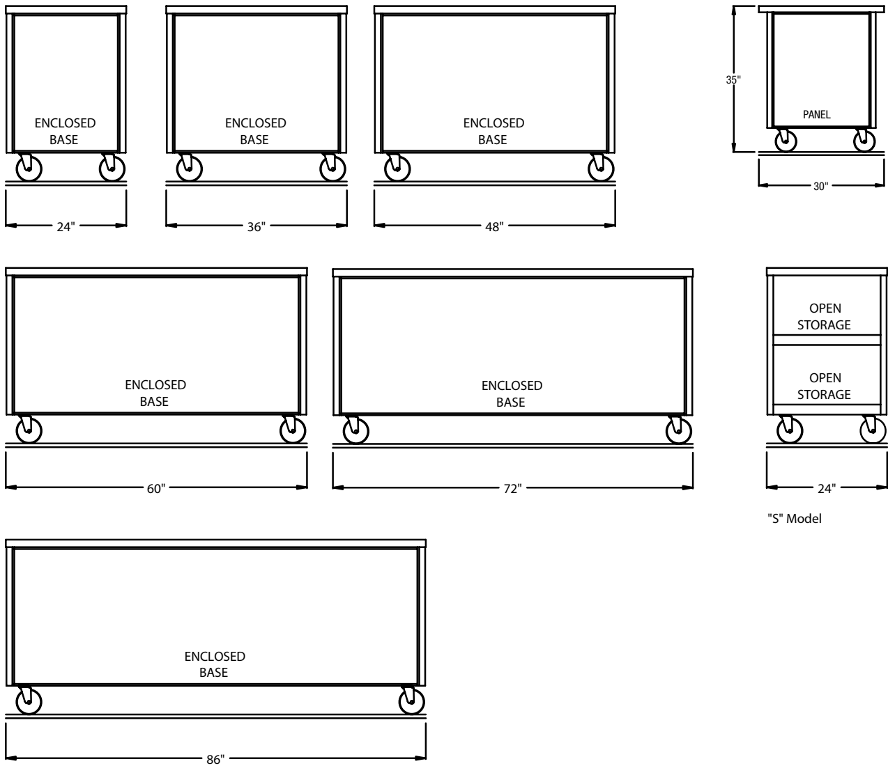
14G ST DRAWINGS SHOWN, 14G ST-S FRONT VIEW SHOWN AS REPRESENTATION OF "S" MODELS Drawings are to be viewed in the same order as the chart
