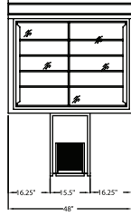
DROP-IN PASS-THRU DISPLAY CASE W/GLASS DOORS ON BOTH SIDES
