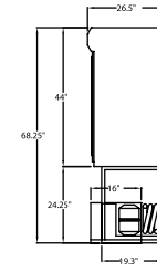
DROP-IN SINGLE SERVICE DISPLAY CASE W/GLASS DOORS & FULL GLASS BACK
