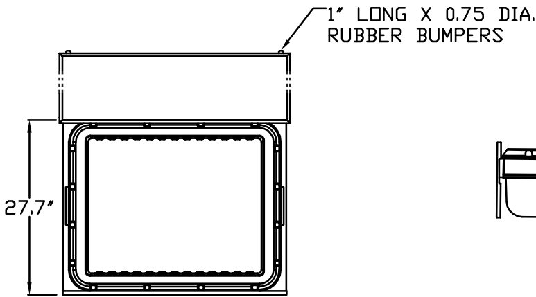
TOP VIEWS
