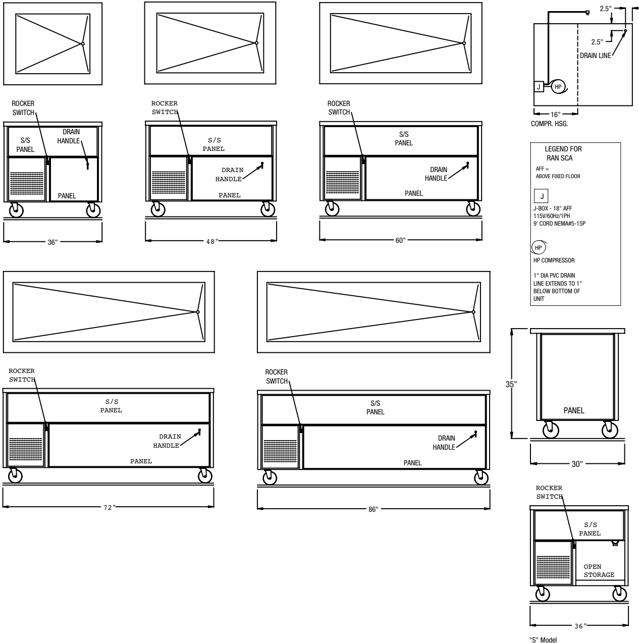
RAN SCA DRAWINGS SHOWN, RAN SCA-S FRONT VIEW SHOWN AS REPRESENTATION OF "S" MODELS Drawings are to be viewed in the same order as the chart
