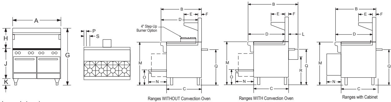
Dimensions - in(mm)
