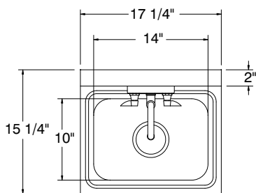
TOP VIEW FOR 7-PS-40 & 7-PS-66
