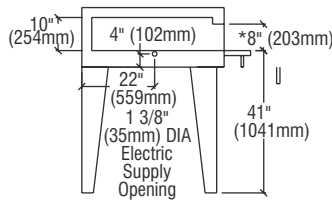
EP-EB-8-3836 SIDE VIEW
