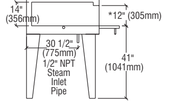
ER-12-3836 SIDE VIEW
