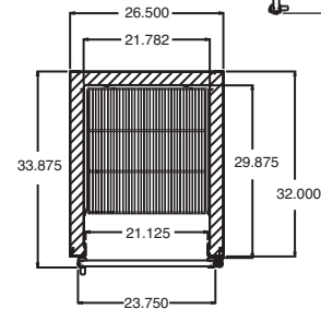
Plan Views
