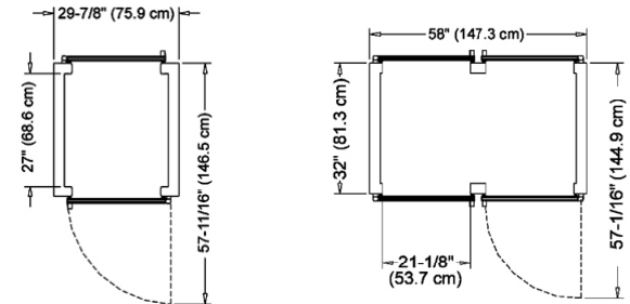
Plan - R/AHT132WPUT
