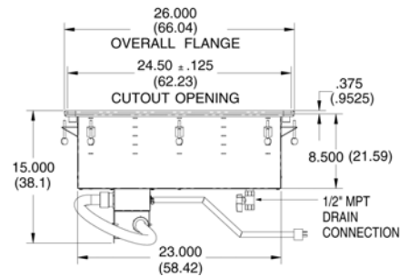
Standard Drain
