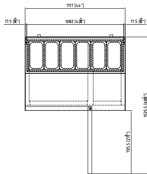
TOP VIEW FBPT44
