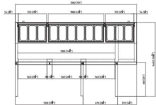
TOP VIEW FBPT93
