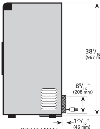
RIGHT VIEW
