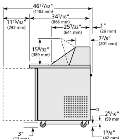
RIGHT VIEW
