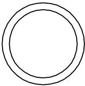
001062-45 O-RING 11/16" I.D. [17mm] 3/4" O.D. [19mm] ( 2 SUPPLIED )
