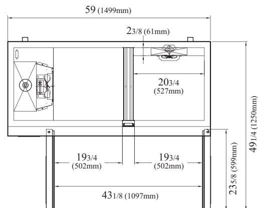
PLAN VIEW
