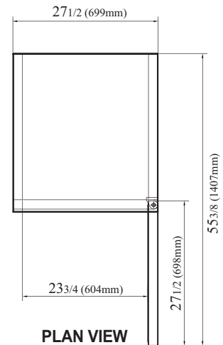
PLAN VIEW
