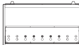
Covered TOM-50 Plan View
