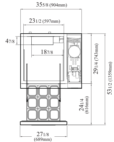
PLAN VIEW
