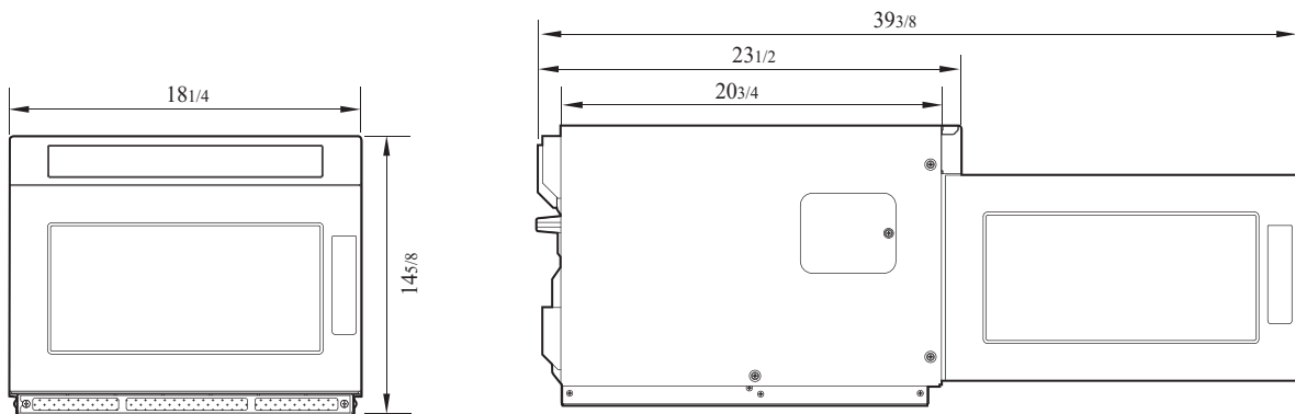
FRONT VIEW
