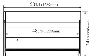
TOM-50S(B) TOP VIEW
