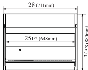
TOM-30S(B) TOP VIEW
