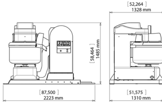
SL120LB
