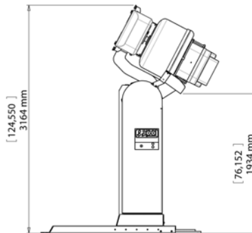
SL120LH
