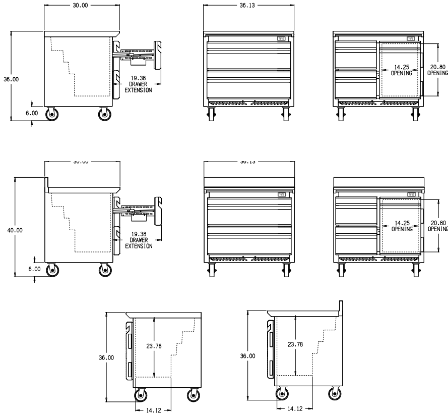
Dimensional tolerances +/- 1/4". Metric dimensions (MM)
