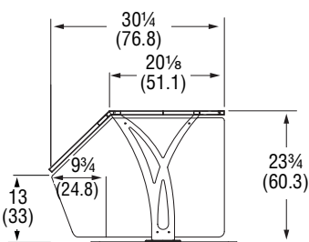
Single-Sided Buffet with Top Shelf – NSF
