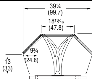
Double-Sided Buffet NSF
