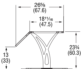
Single-Sided Buffet with Top Shelf – Standard
