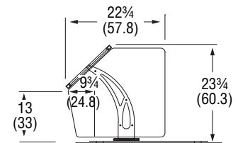
Single Sided Buffet NSF
