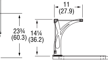
Cafeteria with Top Shelf Standard
