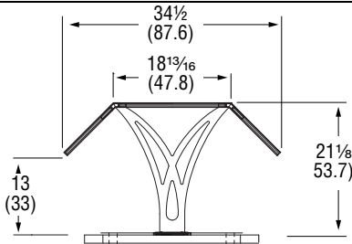
Double-Sided Buffet Standard
