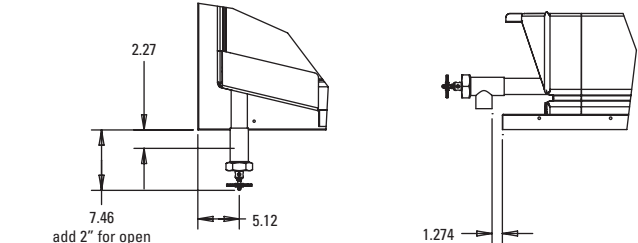
2" Draw-off valve – left front straight (BPD0V-1)
