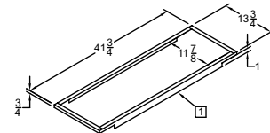
ADAPTER BAR
